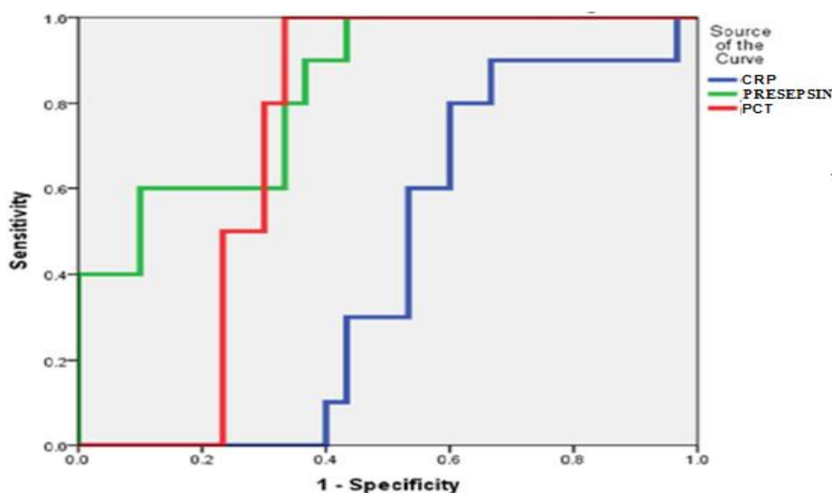
Fig. 2. ROC curve
